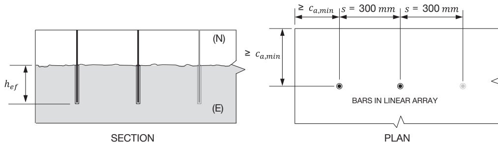
Figure 12 — Illustration of Table 67 dimensions
