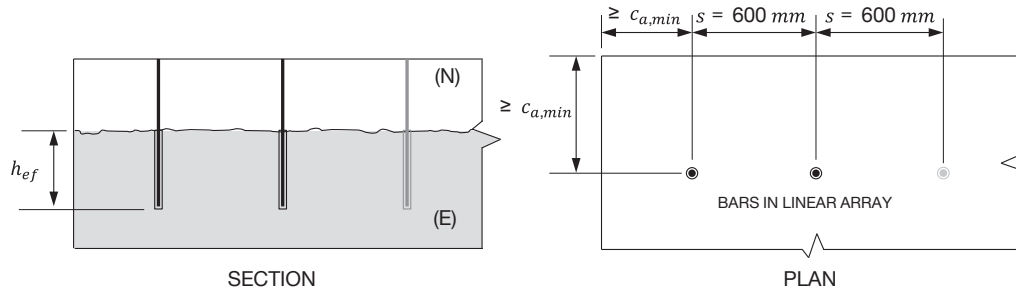
Figure 10 — Illustration of Table 65 dimensions
