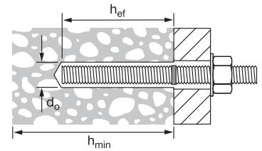
Figure 3 — HAS threaded rods
