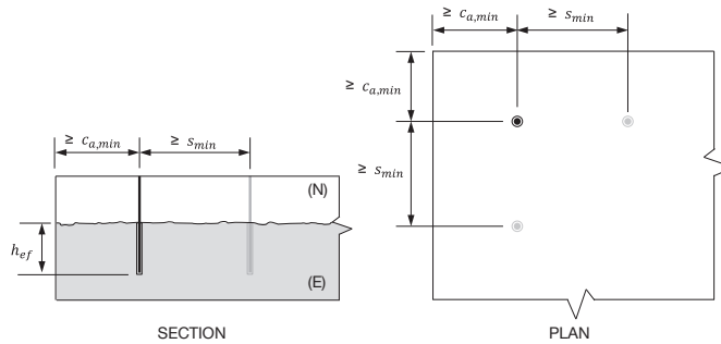
Figure 6 — Illustration of Table 60 dimensions
