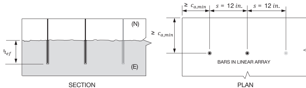
Figure 9 — Illustration of Table 63 dimensions
