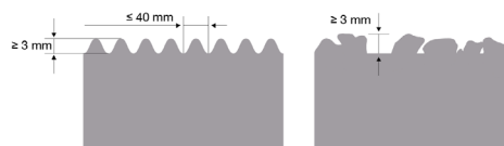
Fig. 9.2: Surface roughness requirement
