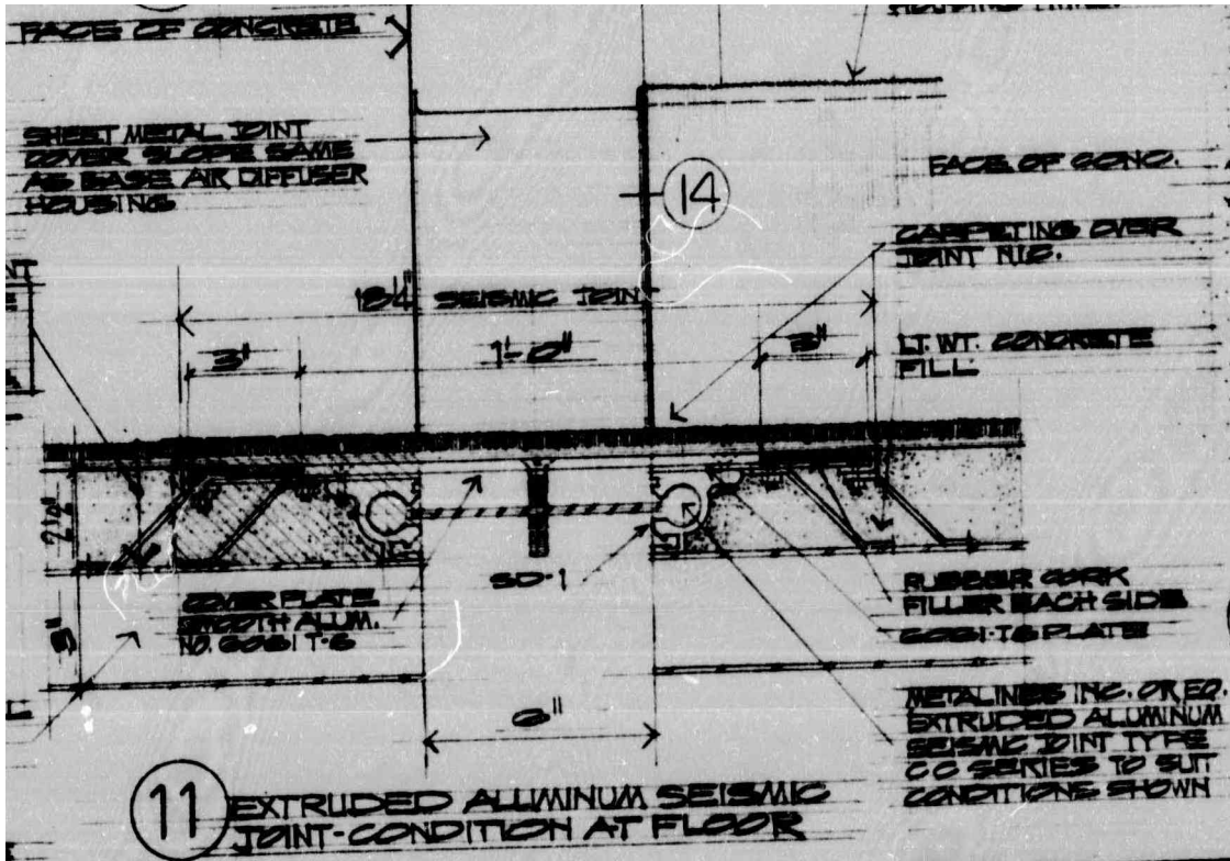
ORIGINAL CONSTRUCTION
