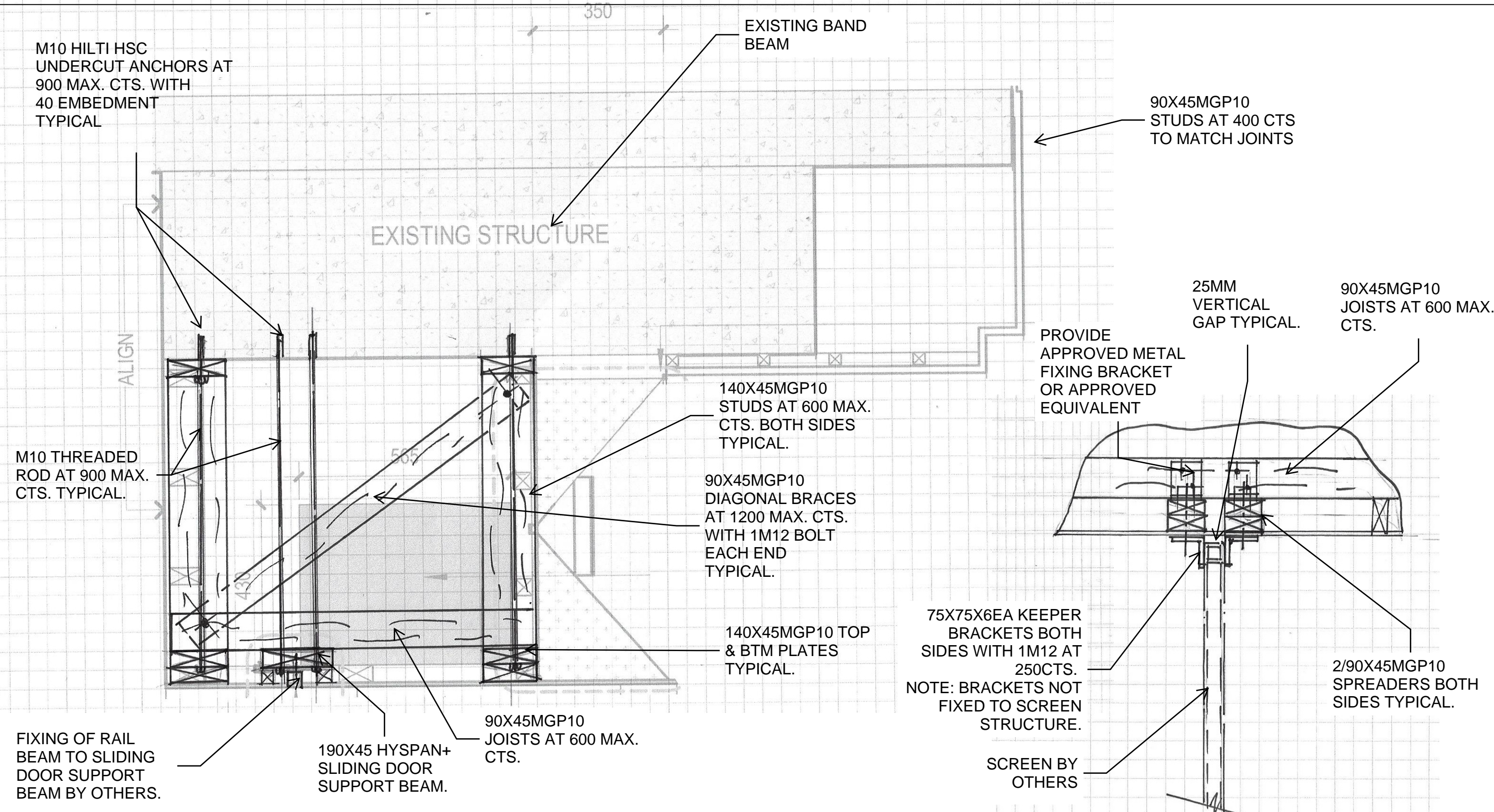
TYPICAL SHOPFRONT BULKHEAD SECTION
