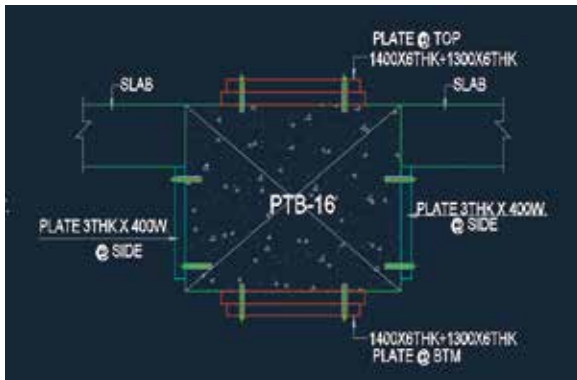
(b) PT beam strengthening details
