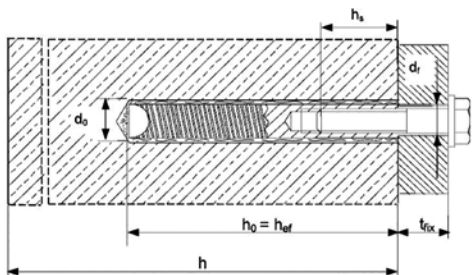
Figure A3: Internally threaded sleeve HIS-(R)N
