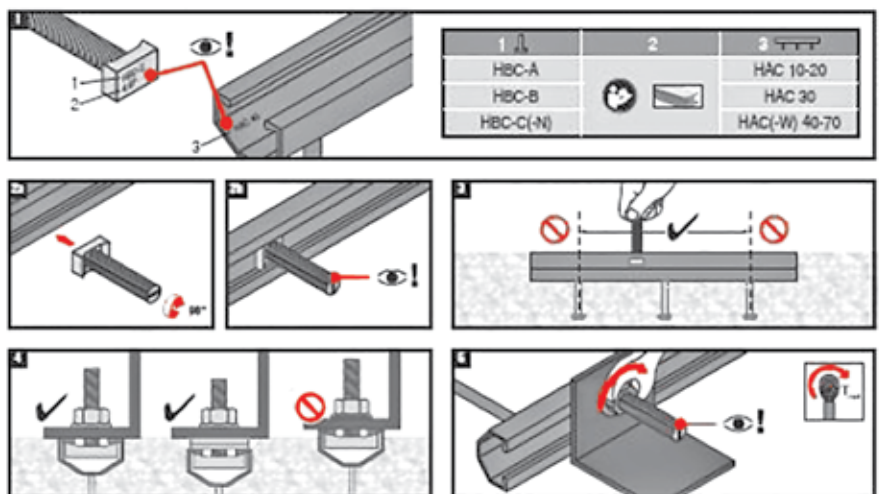
(b) Installation of channel bolt
