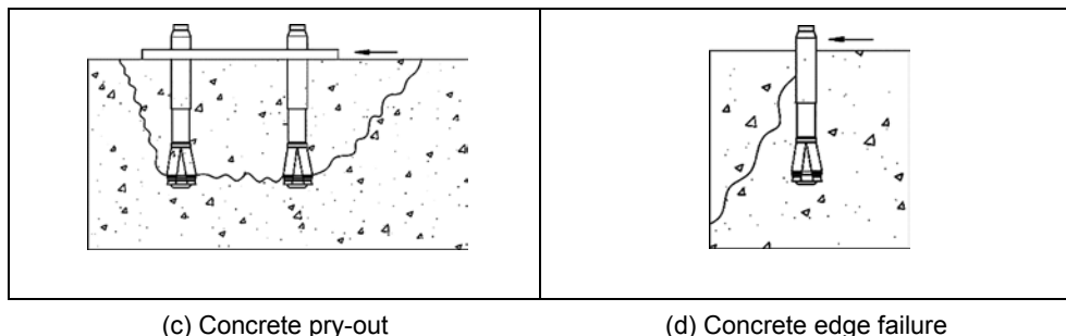
Fig.3.9 Probable failure modes of post-installed anchors in shear [6]
