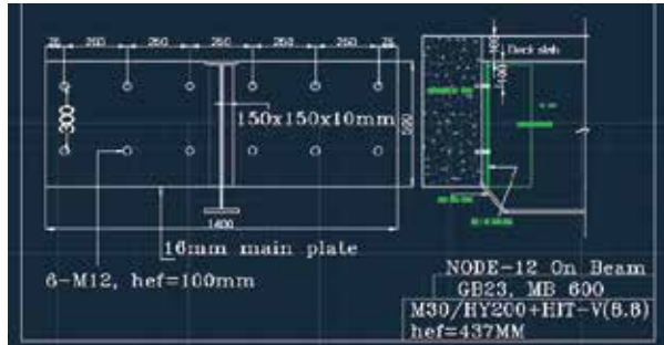
(a) ISMB fixing connection details
