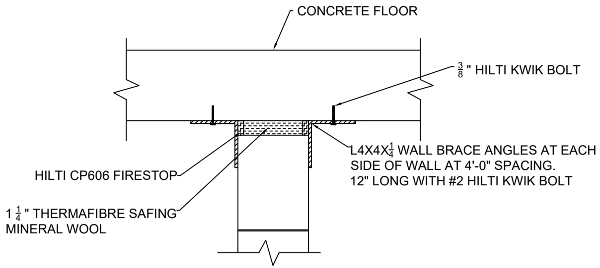
SECTION A-A TYPICAL HEAD OF WALL DETAIL
