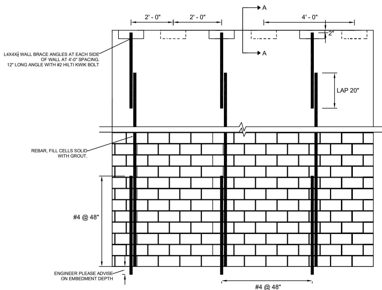
TYPICAL INTERNAL WALL ELEVATION
