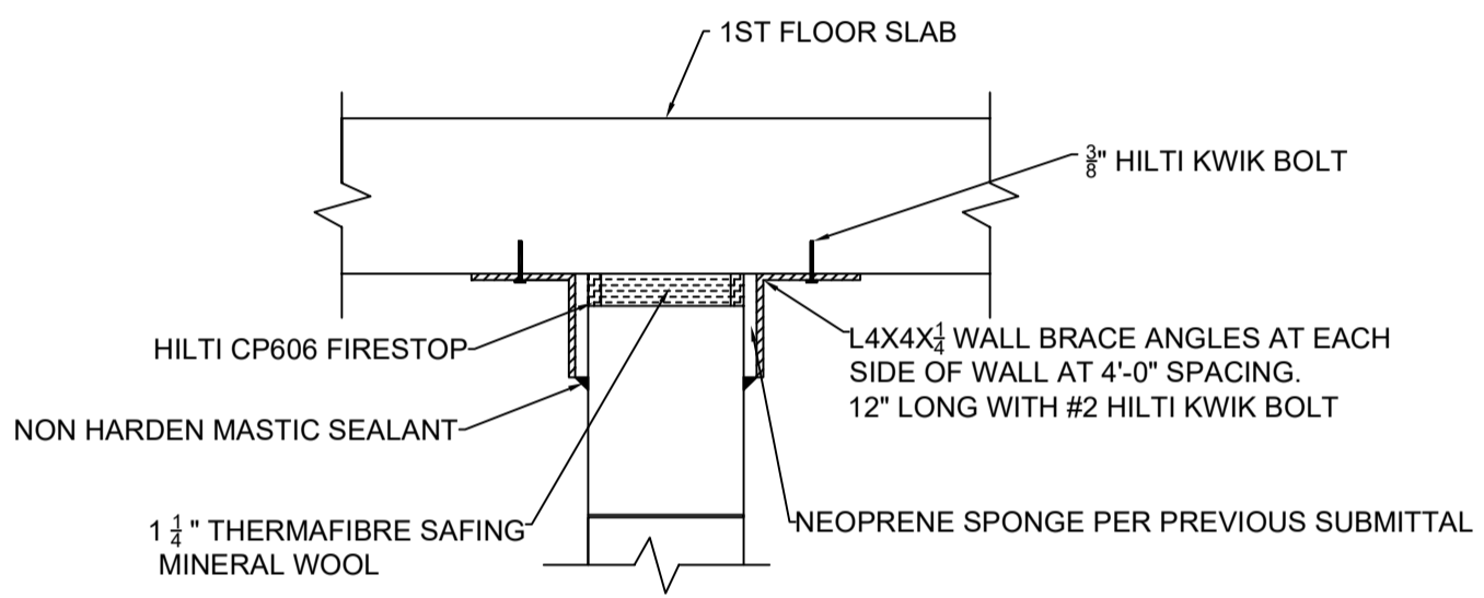
HEAD OF WALL AT ISOLATED PORTION OF FIRST FLOOR SLAB
