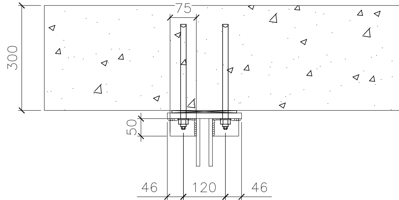
FRONT VIEW A-A
