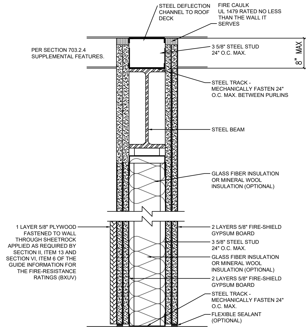
PARTITION - 2 HR UL DESIGN: U411
