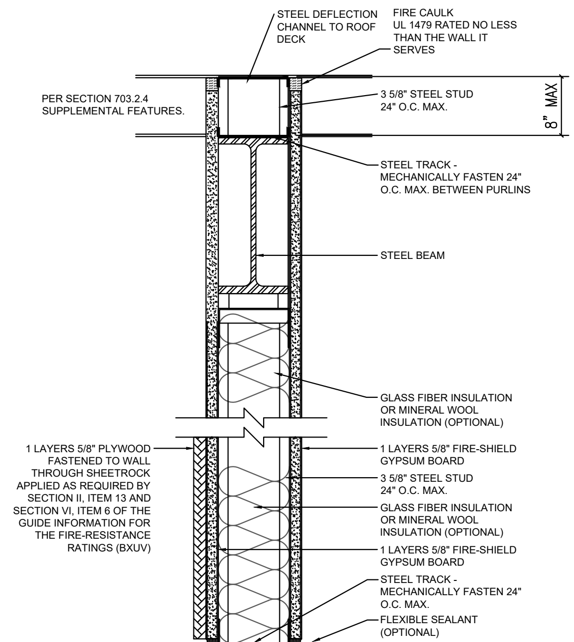
PARTITION - 1 HR UL DESIGN: U419
