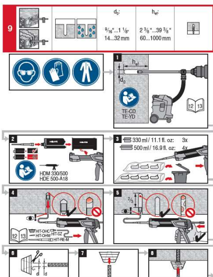
FIGURE 9A—MANUFACTURER'S PRINTED INSTALLATION INSTRUCTIONS (MPII) (Continued)
