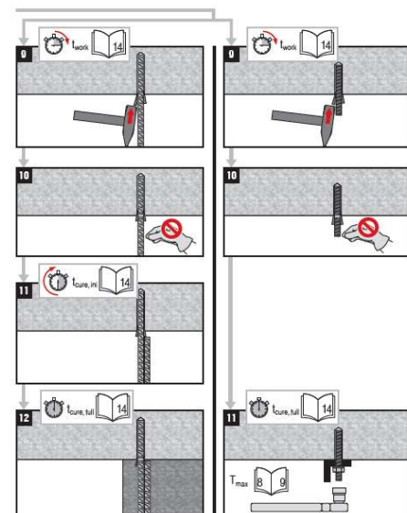
FIGURE 9A—MANUFACTURER'S PRINTED INSTALLATION INSTRUCTIONS (MPII) (Continued)
