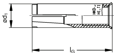
Anchor body
