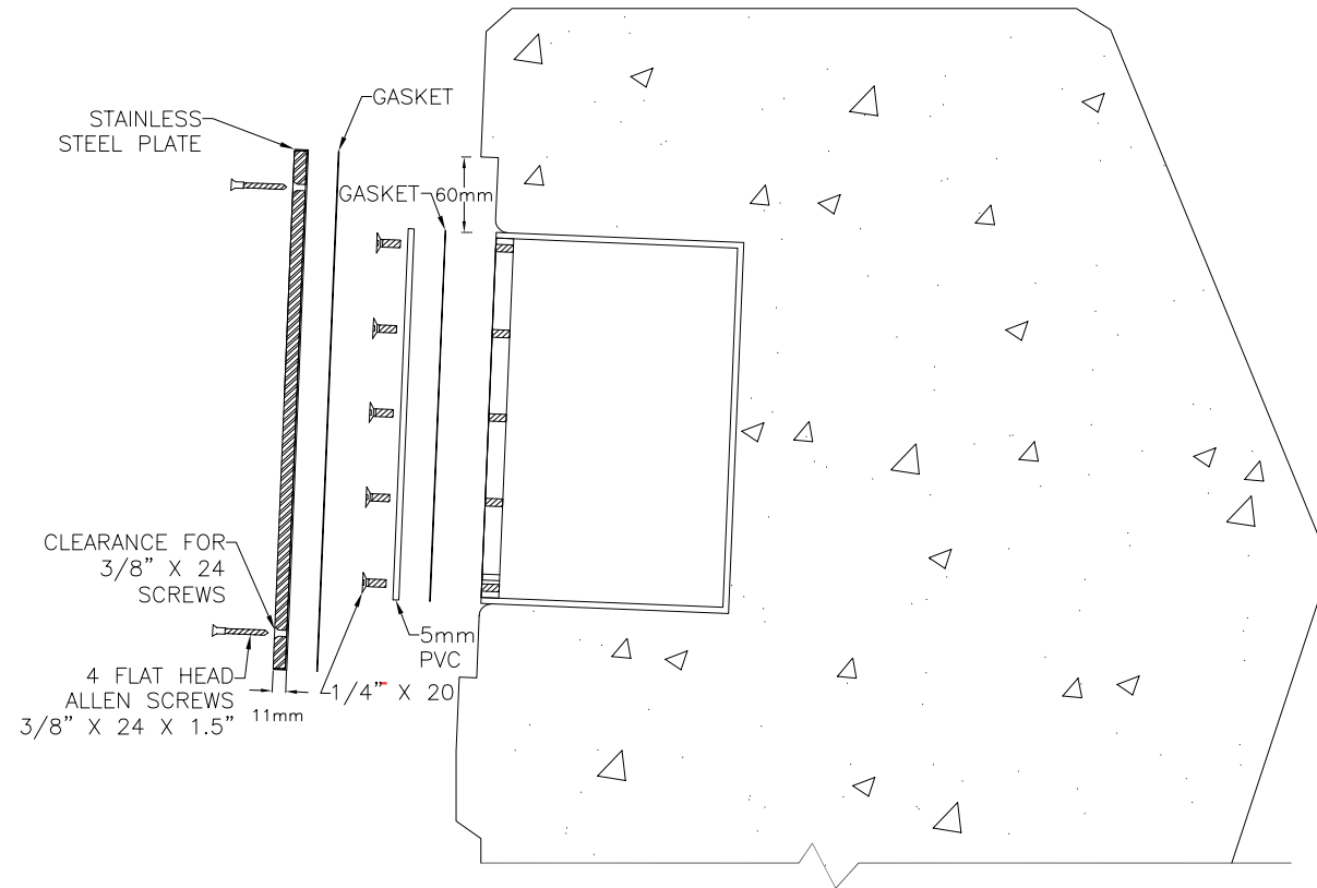
STAINLESS STEEL PLATE INSTALLATION DETAILS
