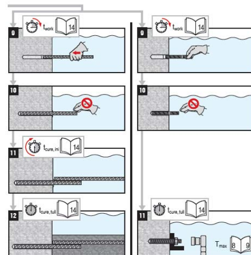
FIGURE 9A—MANUFACTURER'S PRINTED INSTALLATION INSTRUCTIONS (MPII) (Continued)
