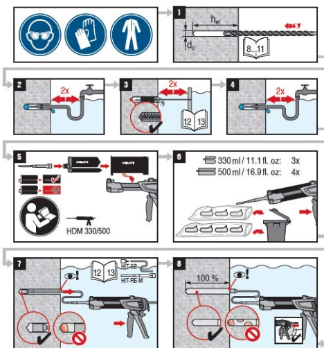
FIGURE 9A—MANUFACTURER'S PRINTED INSTALLATION INSTRUCTIONS (MPII) (Continued)
